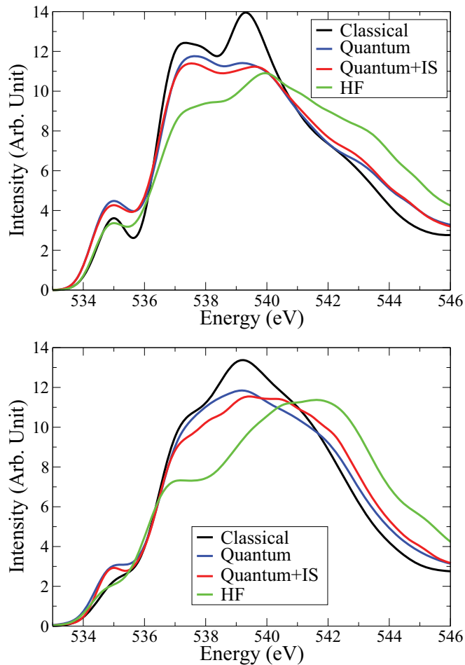
FIG. 1. (Color online) Calculated XAS spectra for liquid water at T = 300 K (top) and ice Ih at T = 269 K (bottom) according to four schemes: (a) COHSEX with classical nuclei and uniform screening (black curve); (b) COHSEX with quantum nuclei and uniform screening (blue curve); (c) COHSEX with quantum nuclei and inhomogeneous screening (IS) (see text; red curve); and (d) Hartree-Fock with quantum nuclei (green curve). Spectra are area normalized and Gaussian broadened (FWHM = 0.4 eV). In order of increasing energy, three features, the pre-edge, the near edge, and the postedge, characterize the spectra.
