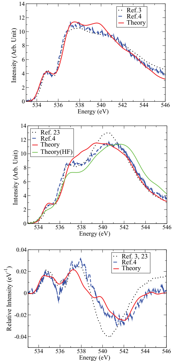
FIG. 2. (Color online) Comparison of calculated XAS spectra with experiments for water (top), ice Ih (middle), and the difference between water and ice Ih (bottom). Two sets of experimental data are included for each system. 3,4,23 Hartree-Fock (HF) data on ice have also been included for comparison (see discussion in the text). Water is at room temperature in theory and experiments, ice is at T = 269 K in the present calculation, at T = 130 K in Ref. 23, and at T = 40 K in Ref. 4. The difference spectrum is obtained from [I(\text{water}) - I(\text{Ih})]/S , where I denotes the spectral intensity and S is the integrated area of the spectra in the energy range of the figure.
