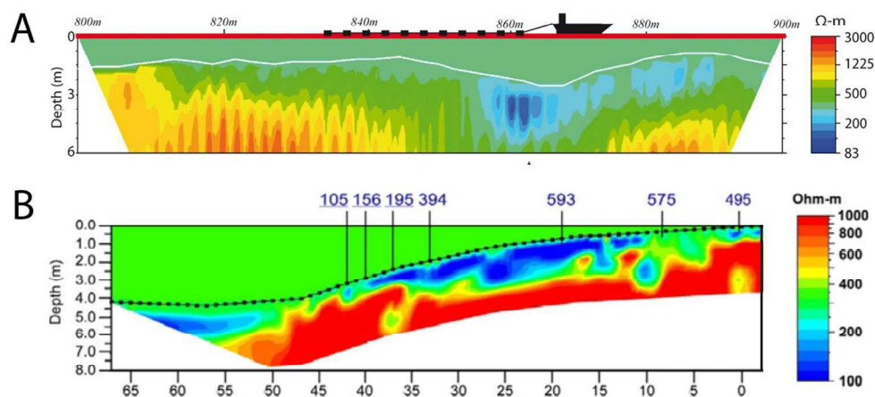
Figure 5: A plume of groundwater contaminated by road salts was revealed beneath Mirror Lake in NH using geophysical surveys. Two perpendicular cross sections are shown. A. The towed resistivity survey around the circumference of the lake showed a high conductivity region in blue. B. The length of the plume perpendicular to the shore was then delineated by a lake bottom resistivity survey. The plume was confirmed by chloride concentrations in water collected from seepage meters. Chloride concentrations from 105 to 593 are shown in units of \mu\text{eq/L} . The lake concentration was 104 \mu\text{eq/L} . The conductive zone from 55 to 65 m in the deep part of the lake is organic sediments.
