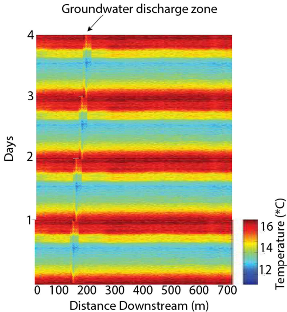
Figure 8: Hypothetical distributed temperature system (DTS) data showing the spatial and temporal resolution. Along the vertical axis is the variation in time over 4 days, which shows a diurnal temperature signal. Along the horizontal axis is a 700-m-long survey. In this hypothetical diagram a groundwater discharge zone indicated by a shift in temperature (cooler in day and warmer at night) is shown around 150 m. This zone drifts slightly downstream to 200 m over the course of the monitoring (artificially generated offset in the temperature shift).
