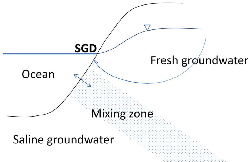
Figure 3: Submarine groundwater discharge (SGD) provides freshwater and dissolved solids to the ocean. SGD occurs along the shore driven by head in aquifers. A mixing zone of freshwater and seawater occurs at the boundary between saline and freshwater, and flow directions can be both into and out from the ocean.
