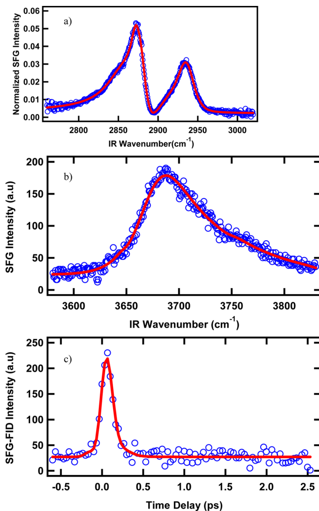
Figure 1. (a) SFG spectrum of ODS-coated silica interface in contact with H 2 O in the C–H stretching region. (b) SFG spectrum and (c) SFG-FID of ODS-coated silica interface in contact with H 2 O in the free O–H stretching region (~3700 cm -1 ). The polarization combination for SFG, vis, and IR is S,S,P.
