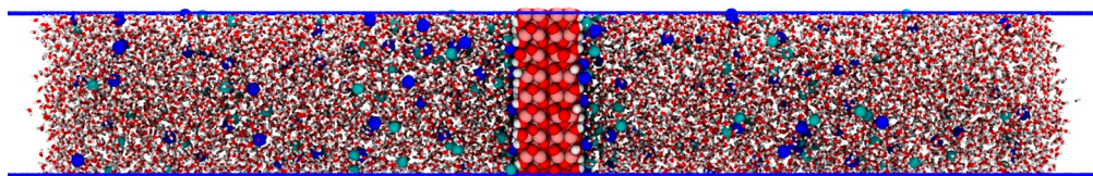
Figure 1. Snapshot of the classical MD simulation box. The simulation box is symmetric with the alumina in the middle. Two water–air interfaces are created to maintain the pressure at that of water–vapor coexistence. The color scheme is as follows: pink, Al; red, O; white, H; blue, Na; green, halide ion.
