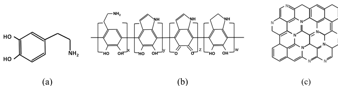
Figure 1. Schematics showing (a) the dopamine molecule, (b) a proposed PDA structure based on covalently bonded linear oligomers. 5 (c) a hypothetical structure of carbonized PDA. 5 Reproduced with permission from ref 5. Copyright 2013 American Chemical Society. Reproduced with permission from ref 9. Copyright 2012 John Wiley and Sons.
