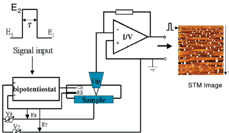
Figure 1. Schematic of potential pulse perturbation time-resolved STM ( P^3 TR-STM). The perturbing pulse raises the sample potential from E_1 to E_2 for a time \tau before returning the sample potential to the potential E_1 . STM monitors the subsequent interfacial dynamics.
