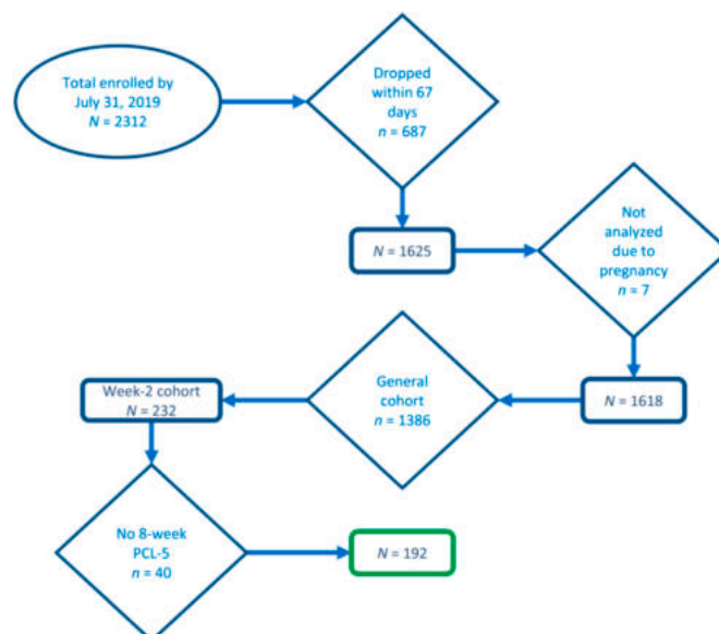
Fig. 1. CONSORT diagram.
